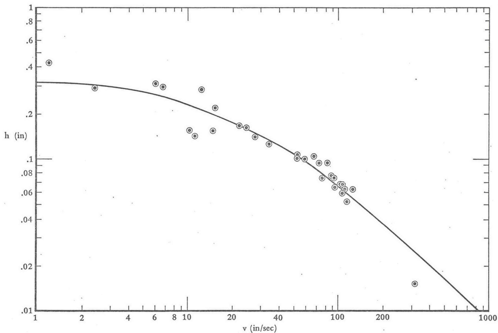
Figure 7. Comparison between experiment and theory for Wilkeson sandstone. The jet impinges normally with a diameter 0.030 inch and a total pressure 17,000 psi. The curve follows from (28) under appropriate assumptions about the parameters.
